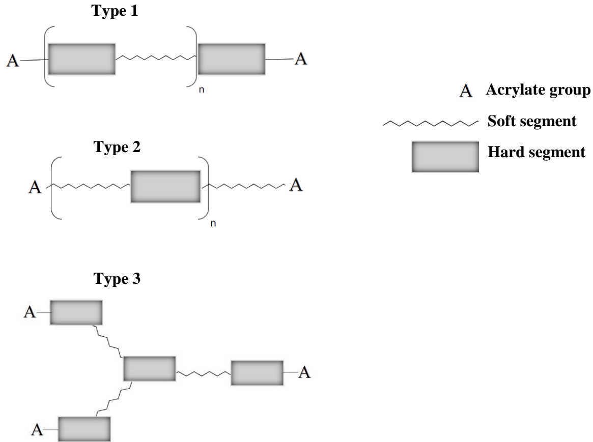
Figure 1. Different Types Polyurethane Acrylates
